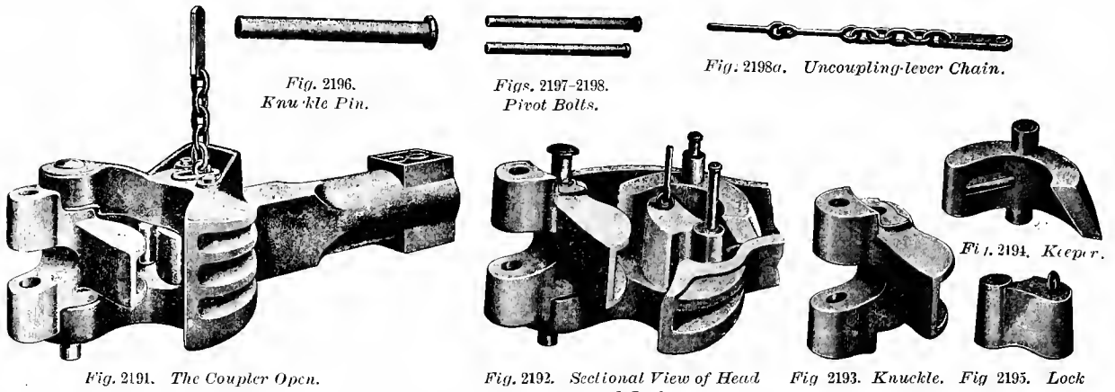
THE POOLEY FREIGHT COUPLER AND PARTS.
